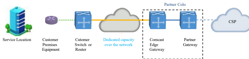
Point-to-cross-connect cloud connectivity service (“P2C”) Point-to-point connectivity between Service Location and cross-connect
